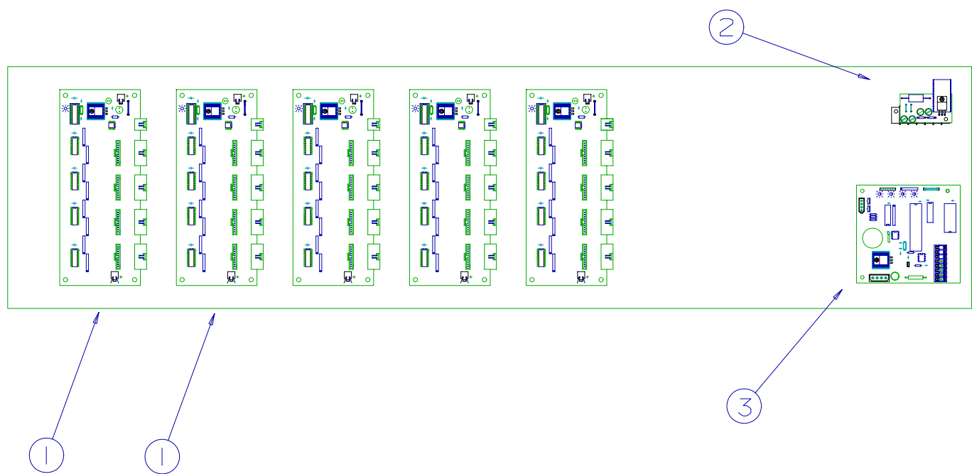
figure 4 CONTROLLER ASSEMBLY
